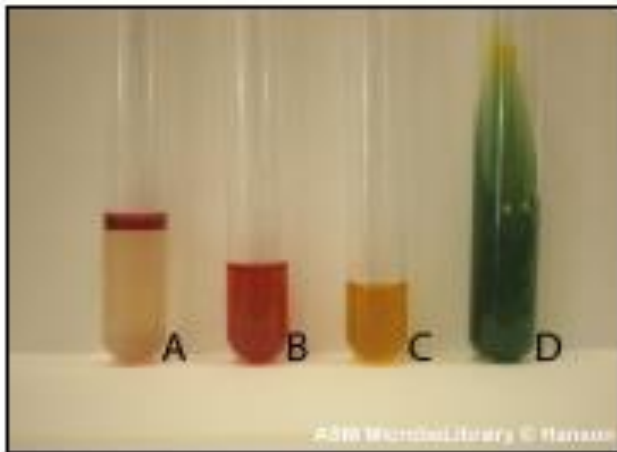
IMViC test
